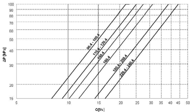
Cold user side exchanger pressure drops
