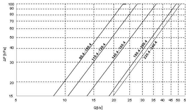
Hot user side exchanger pressure drops
