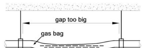
Figure 6.4: Effect of insufficient drain piping support
