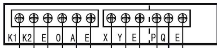
Figure 9.5: Outdoor unit communication terminals
