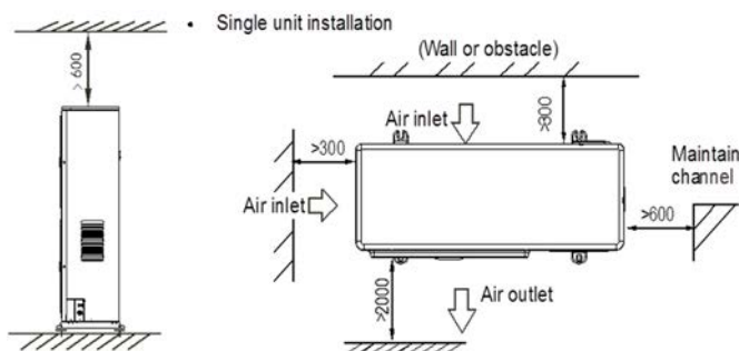
Figure 2.3: Single unit installation [mm]
