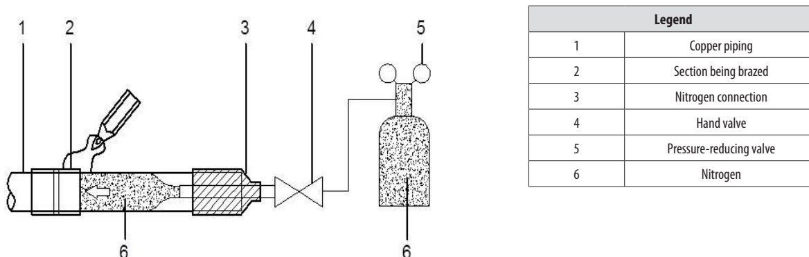
Figure 5.4: Flowing nitrogen through piping during brazing
