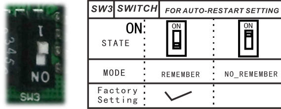
C. Micro-switch SW3 is for selection of auto-restart function. Range: Active, inactive
