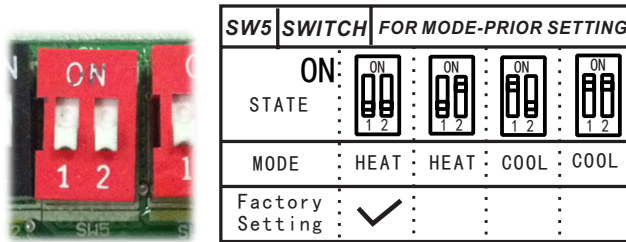
D. Micro-switch SW5 is for setting mode priority of multi connection. Range: Heat, cool.
