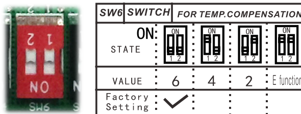
E. Micro-switch SW6 is for selection of temperature compensation in heating mode. This helps to reduce the real temperature difference between ceiling and floor so that the unit could run properly. If the height of installation is lower, smaller value could be chosen. Range: 6°C, 4°C, 2°C, E function (reserved for special customizing)
