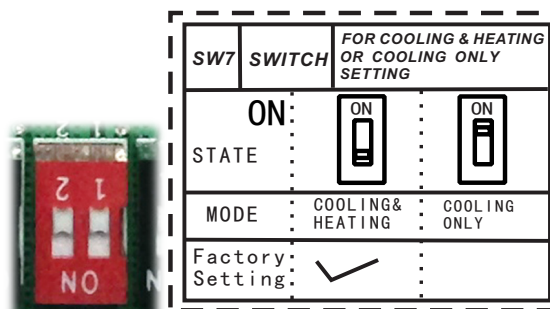
F. Micro-switch SW7 is for setting cooling & heating or cooling only. Range: cooling & heating, cooling.
