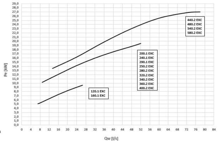
Power input
