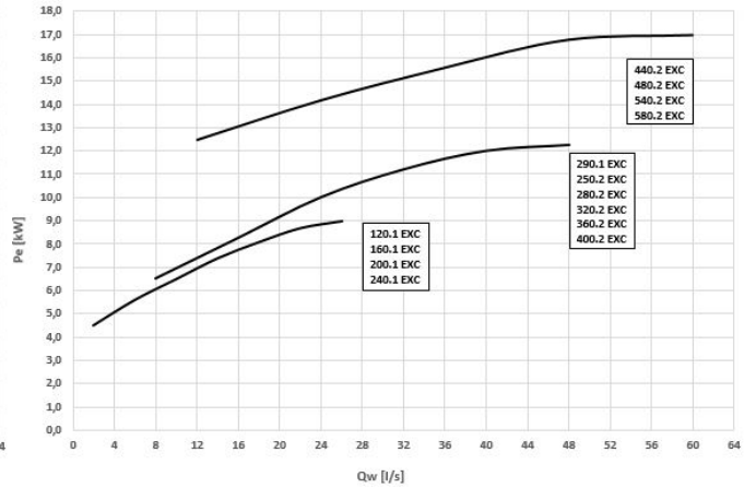
Power input
