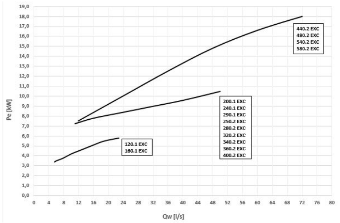
Power input
