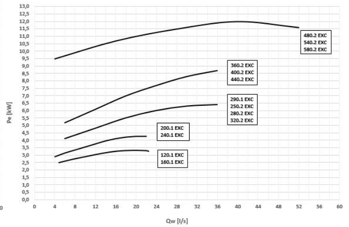
Power input
