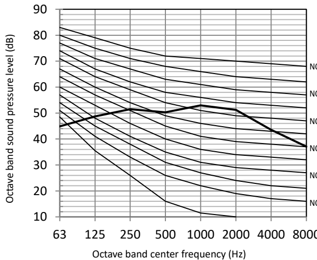
Figure 2-10.6: 160 model octave band level
