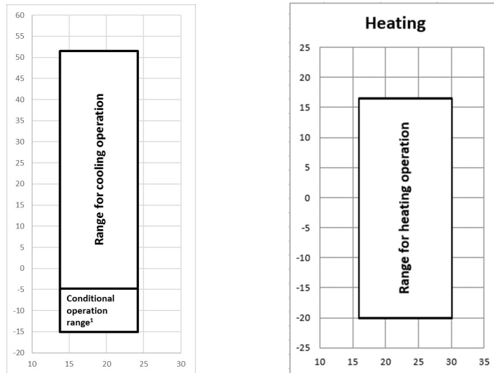
Figure 2-9.1: Operating limits
