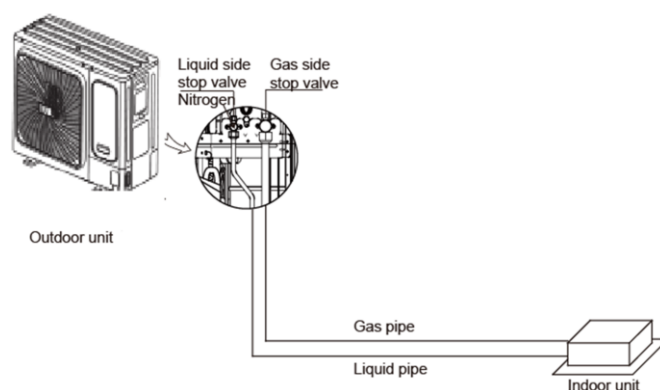
Figure 3-4.16: Gastightness test
