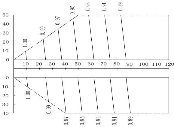
Figure 2-8.11: 120 model rate of change in cooling capacity
