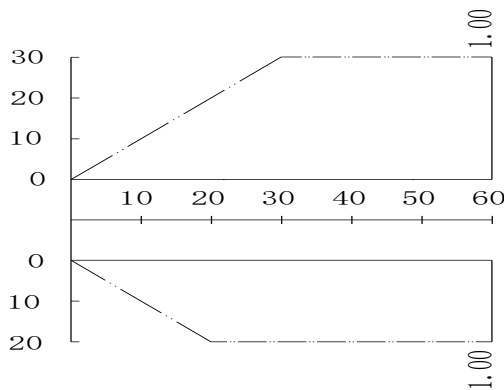
Figure 2-8.6: 120 model rate of change in heating capacity
