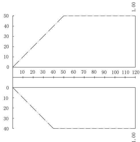
Figure 2-8.8: 140 model rate of change in heating capacity
