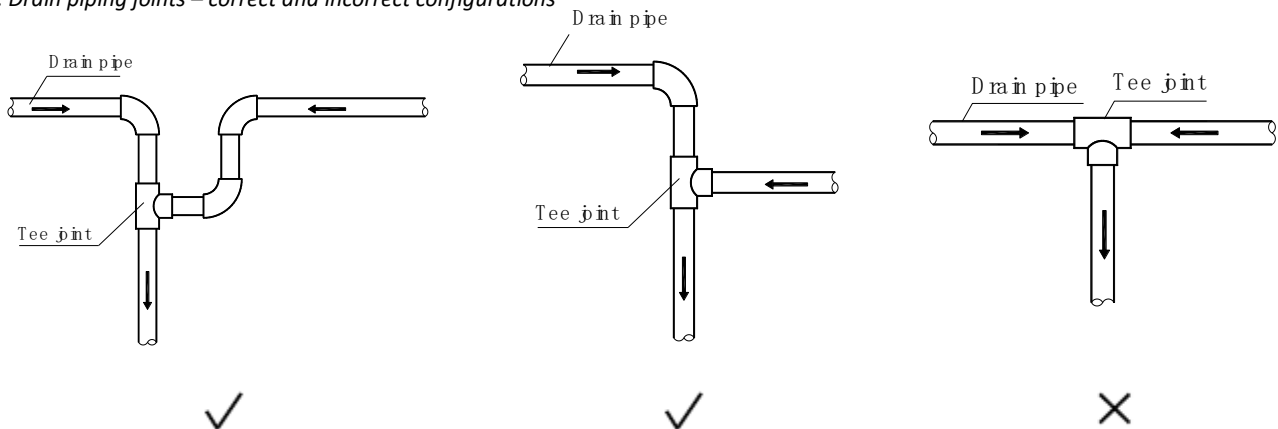
Figure 3-5.2: Drain piping joints – correct and incorrect configurations
