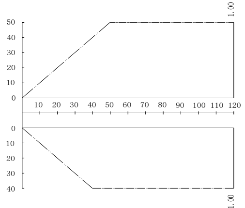
Figure 2-8.12: 120 model rate of change in heating capacity
