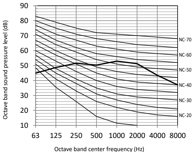
Figure 2-10.5: 140 model octave band level
