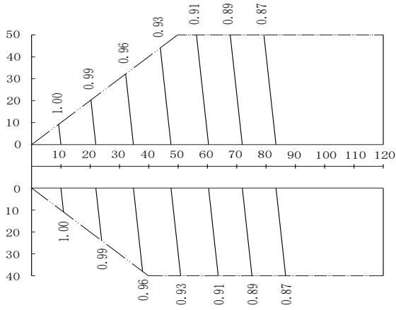
Figure 2-8.15: 160 model rate of change in cooling capacity
