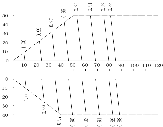
Figure 2-8.13: 140 model rate of change in cooling capacity
