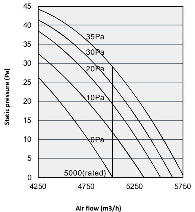
Figure 3-2.6: 120/140/160 model units fan performance
