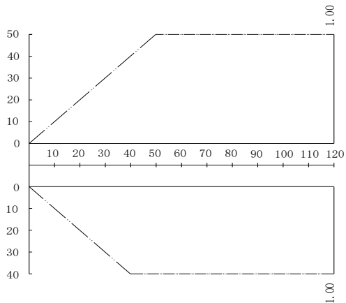
Figure 2-8.8: 140 model rate of change in heating capacity
