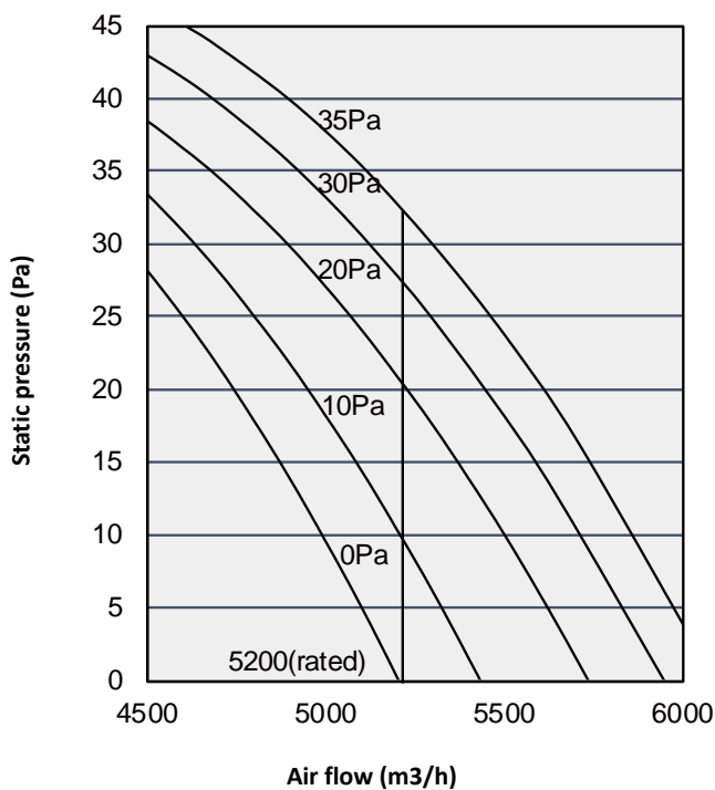
Figure 3-2.5: 80/100 model units fan performance
