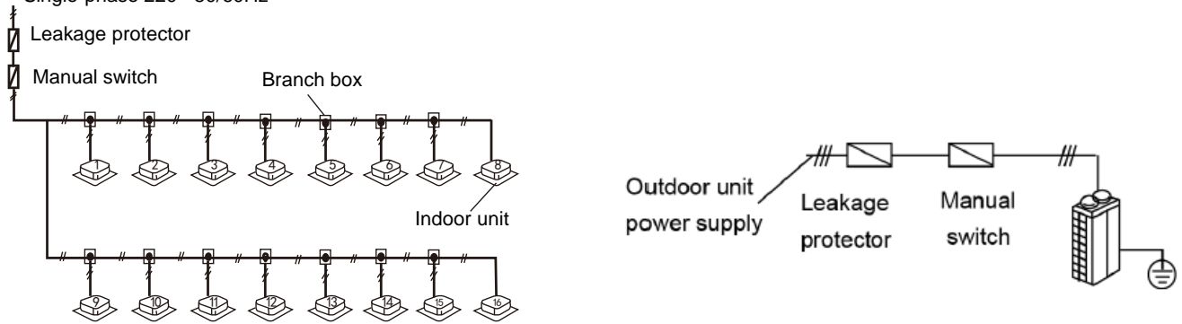
Figure 3-8.1: Indoor unit unified power supply wiring Single-phase 220~ 50/60Hz
