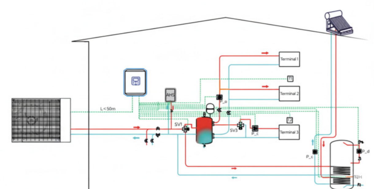
Installation with KITR290X
