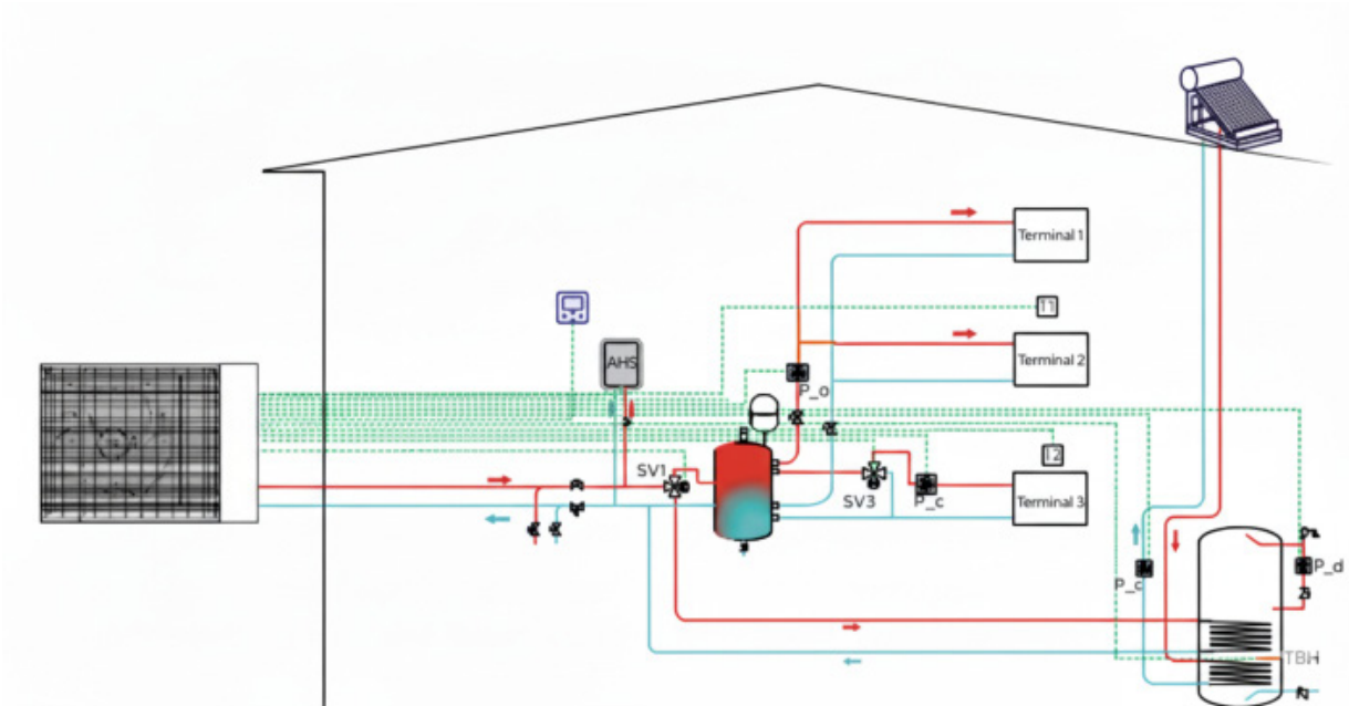
Installation with KITR290X
